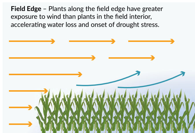
Figure 3. Illustration of the effect of arid wind on the microclimate of the crop canopy.
